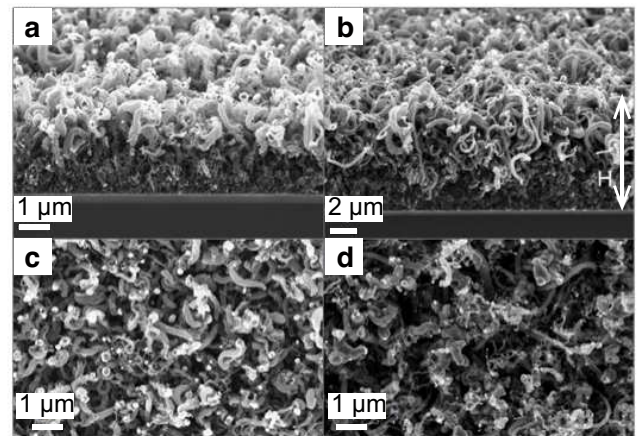
Figure 1: Scanning electron microscope (SEM) images showing side views of the carbon nanofiber (CNF) layers with a synthesis time of (a) 11 min and (b) 14 min. The arrow in (b) indicates the height H of the CNF layer. The corresponding top-view SEM images are shown in (c) for a synthesis time of 11 min and in (d) for a synthesis time of 14 min. The bar represents 1 \mu\text{m} in (a), (c) and (d), and 2 \mu\text{m} in (b).
